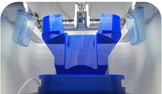
Large flexible parts in TPU 95A to TPU 70A
