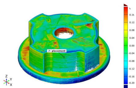
Tested for accuracy We have verified dimensional accuracy within ±0.2 mm or ±0.2% nominal length over the full printer build volume using PPS CF, PET CF, Tough PLA, and PETG.
