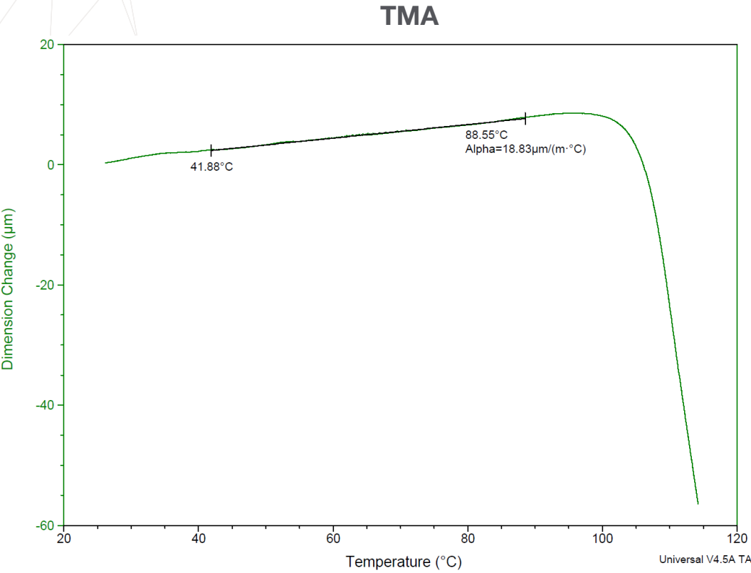
Figure 2. Dimension change data as a function of temperature for ABS-CF10 Flat (XY) sample.
